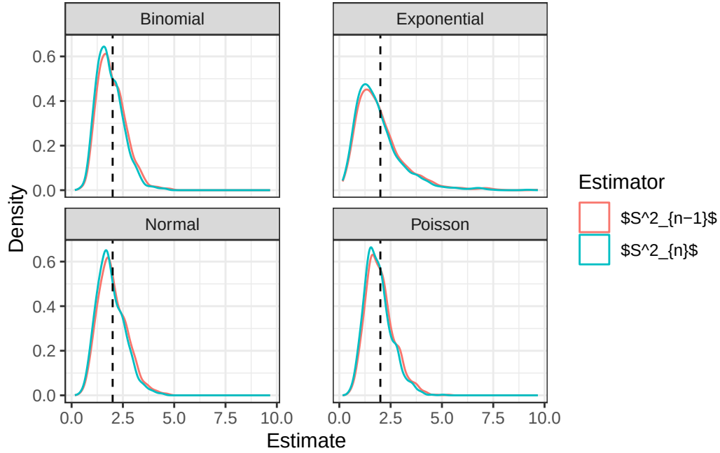
Figure 5: Distributions of Variance Estimators (Boostrapping)
